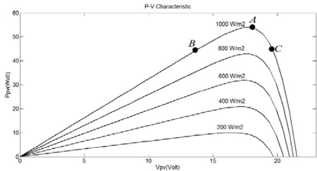
Fig. 4: P-V Characteristics of PV module
