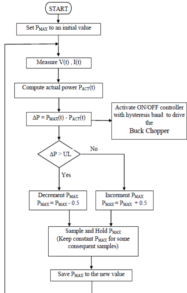
Fig. 5: Flow Chart of the P&O Technique
