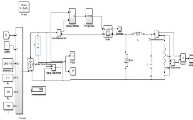
Fig. 10: Overall Simulation circuit
