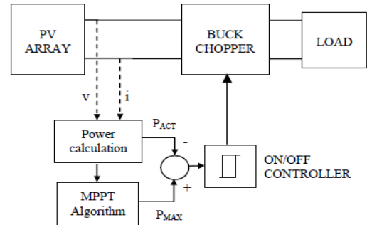
Fig. 7: Block Diagram of the P&O Technique
