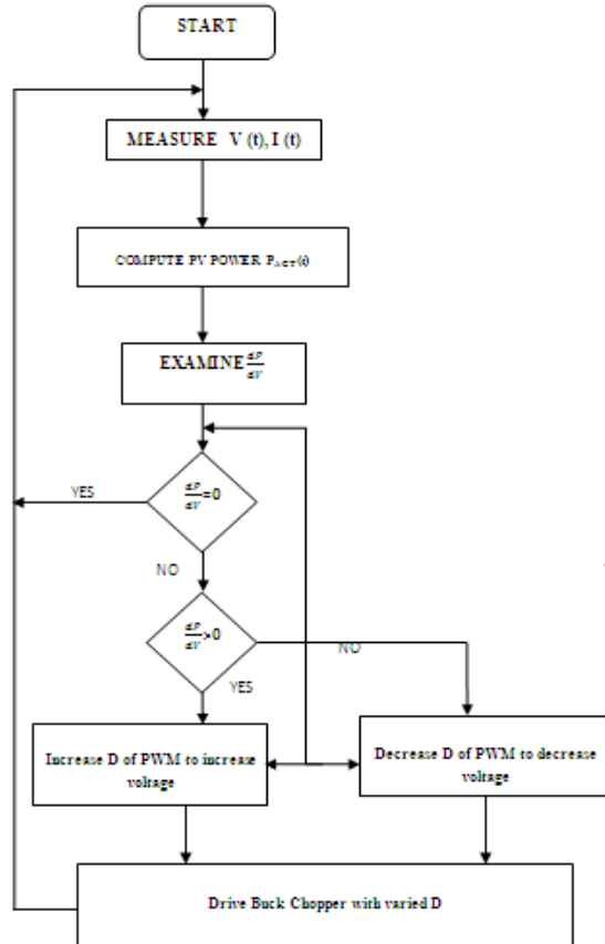
Fig. 6: Flow Chart of the Improved Technique
