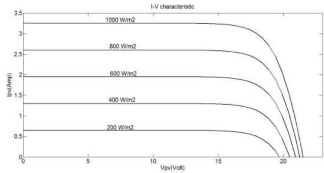
Fig. 3: I-V Characteristics of PV module
