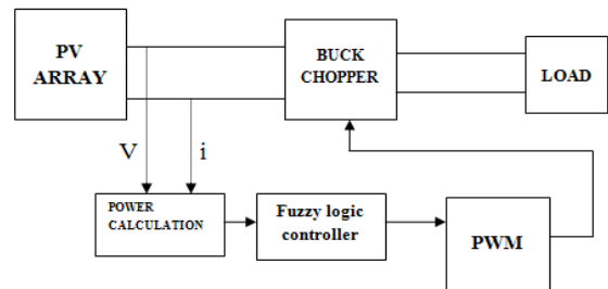
Fig. 8: Block Diagram of the Improved Technique
