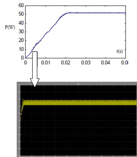
Fig. 9: Tracked maximum power and Extracted PV power before and after improvement
