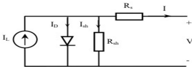
Fig. 2: Equivalent circuit of PV module
