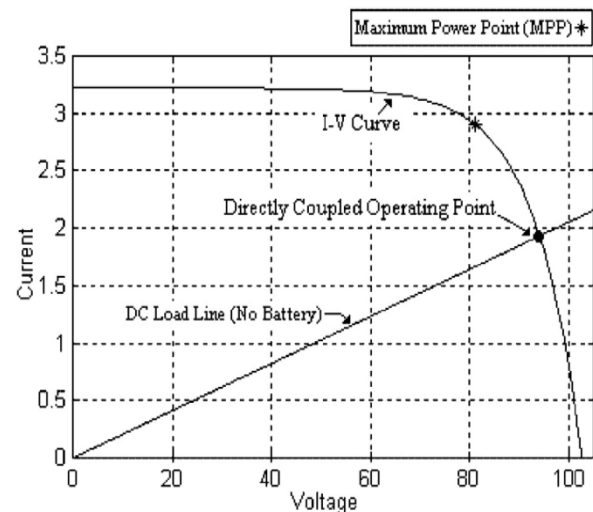
Fig. 1: I-V curve and the load line
